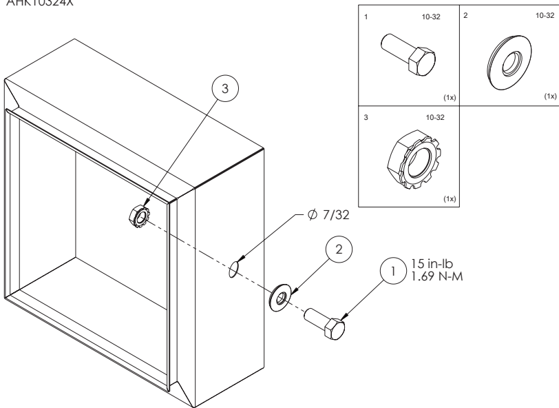
AHK10324X
