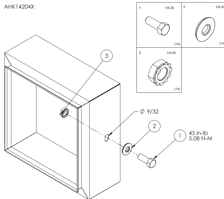
AHK14204X
