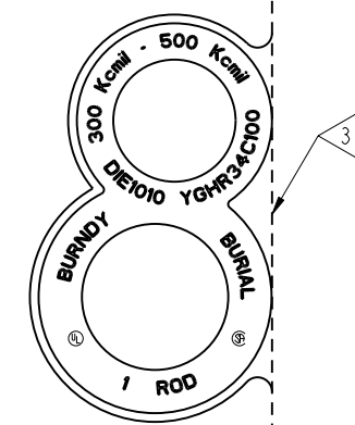
TYPICAL LETTERING
