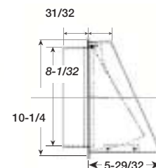
Exterior Hood
